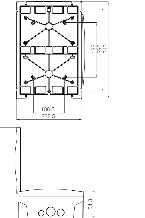
Surface Mount Distribution Box with Terminal Module 16 Double Decker
