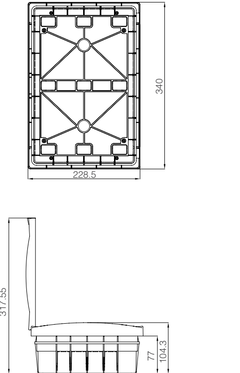
Flush Mount Distribution Box with Terminal Module 16 Double Decker
