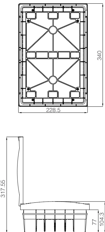
Flush Mount Distribution Box with Terminal Module 16 Double Decker
