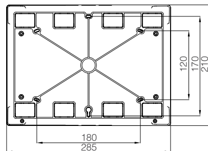
Surface Mount Distribution Box with Terminal Module 12
