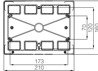
Surface Mount Distribution Box with Terminal Module 8
