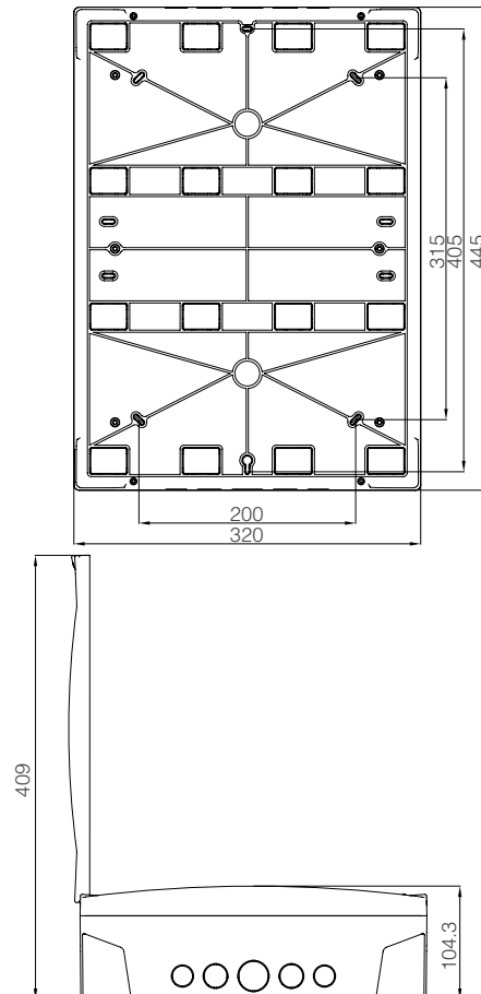
Surface Mount Distribution Box with Terminal Module 36
