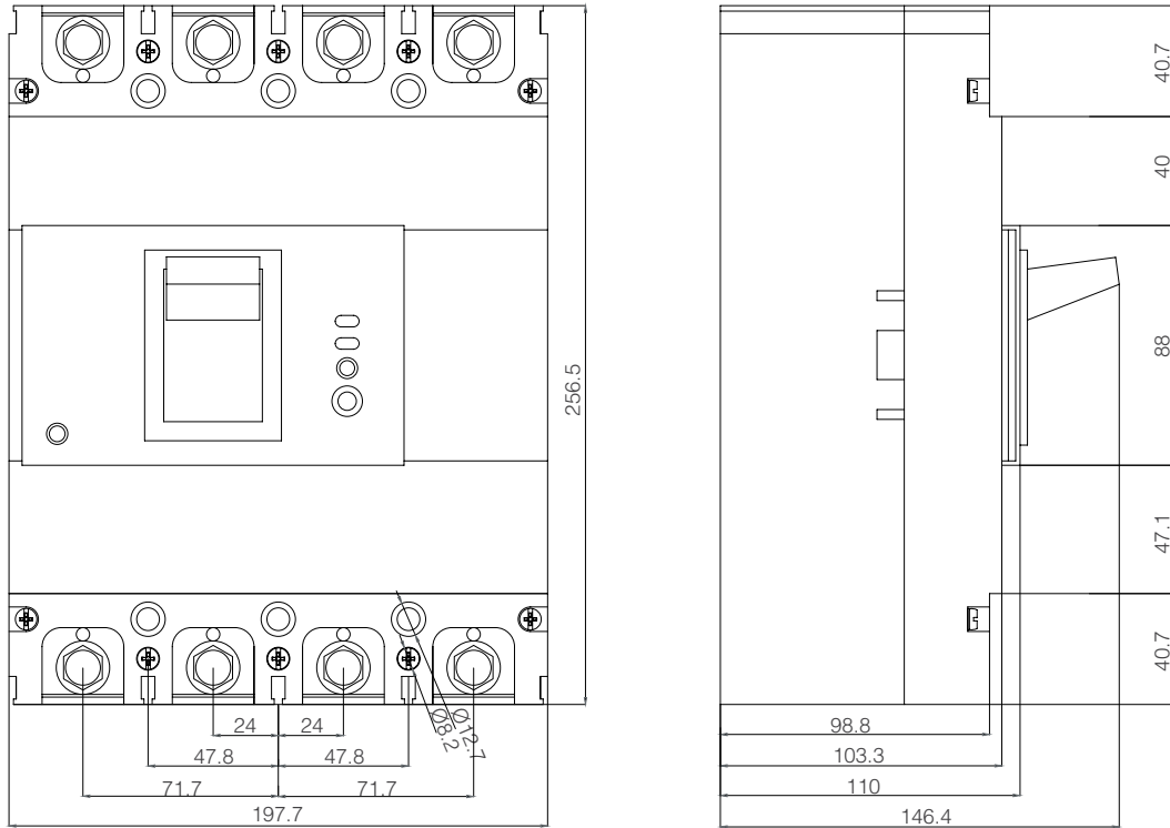
400 A Leak Current Protected Compact Switch
