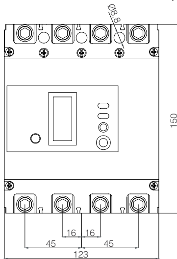
100 A Leak Current Protected Compact Switch
