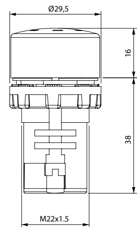
Monoblock Buzzers
