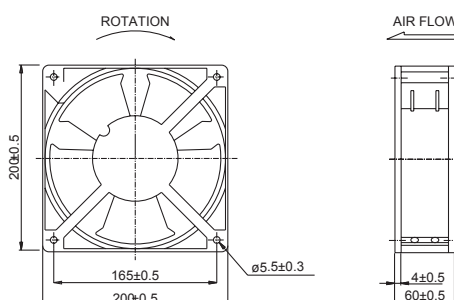
200x200x60
