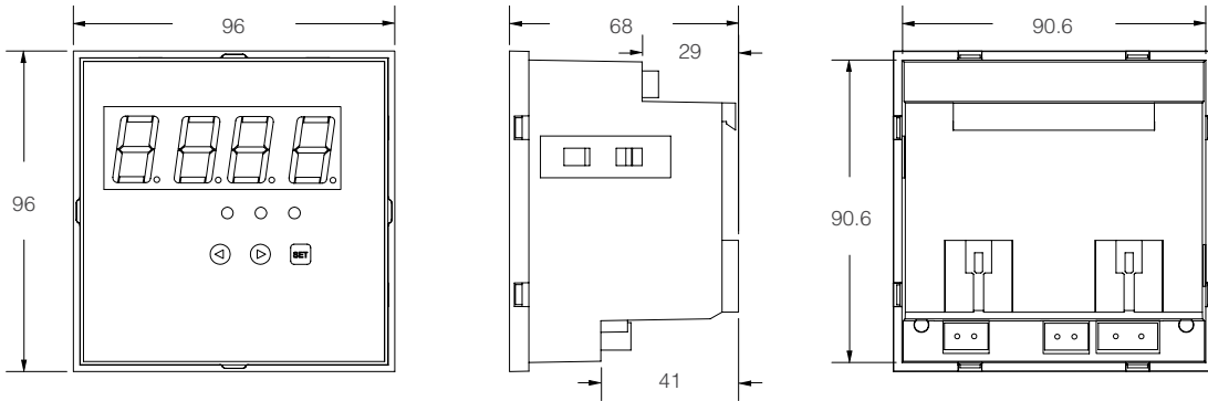
Ampermetre AM1-10
